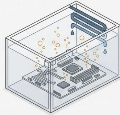
Immersion Cooling
